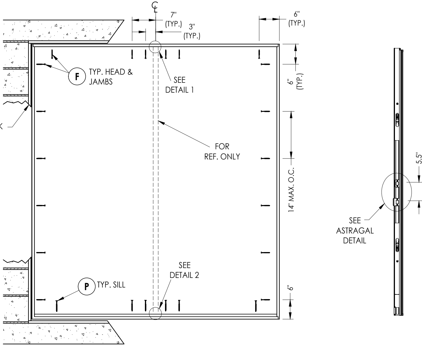
FRAME ANCHORING Masonry 1X buck construction
