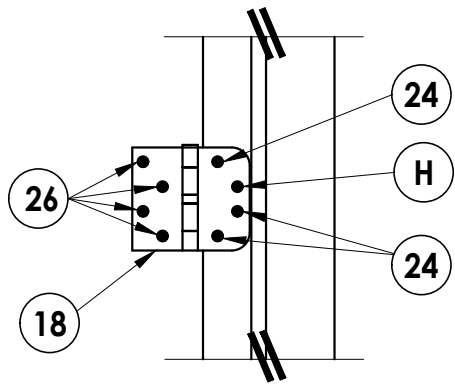
HINGE DETAIL
