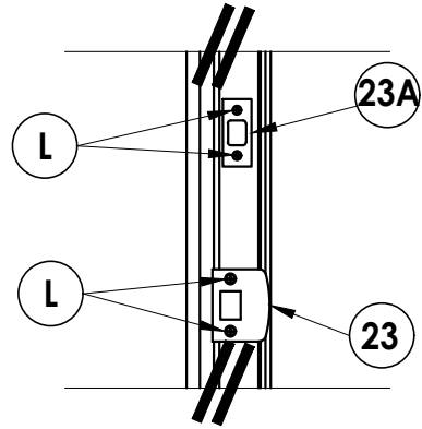
ASTRAGAL DETAIL @ Strike
