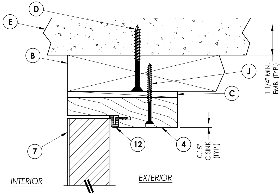
1 4 VERTICAL CROSS SECTION Inswing shown - outswing also approved
